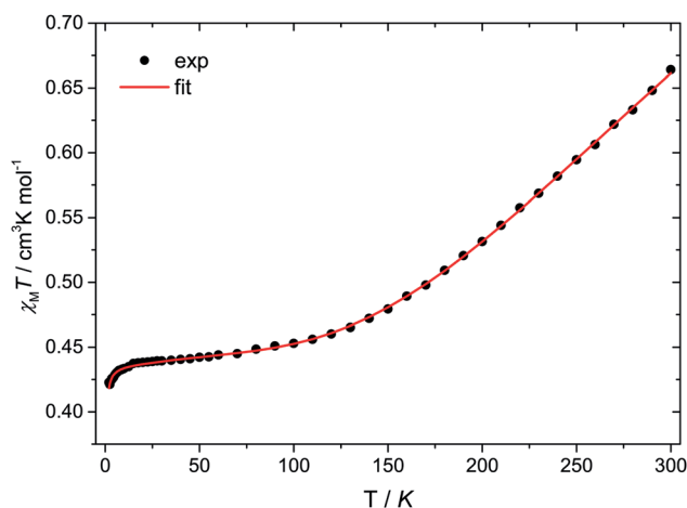
Fig. 2 Temperature dependence of \chi_M T for Cu 3 saltag . The solid red line represents the best fit (see text and Table S6, ESI†).
